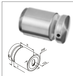
SLAB CONNECTOR
