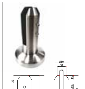
ROUND SPIGOT
