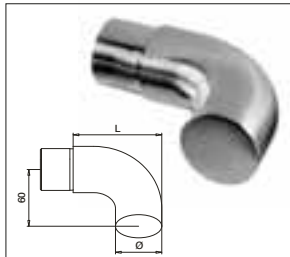
90° TUBE END
