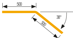
Ramp Bend
