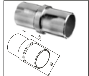
TUBE CONNECTOR
