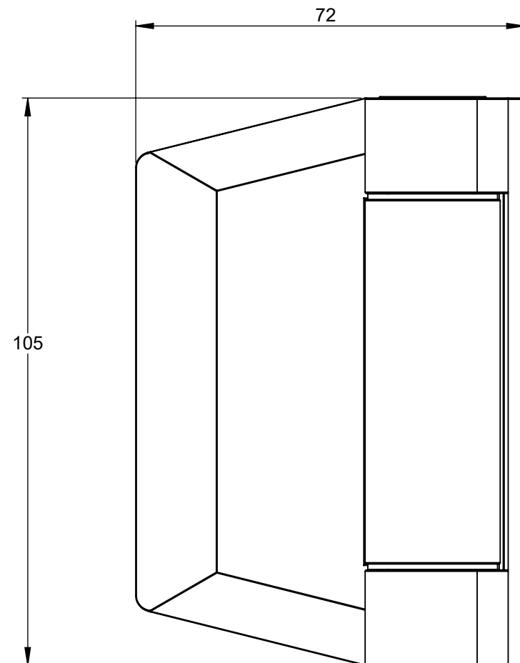
FRONT VIEW
