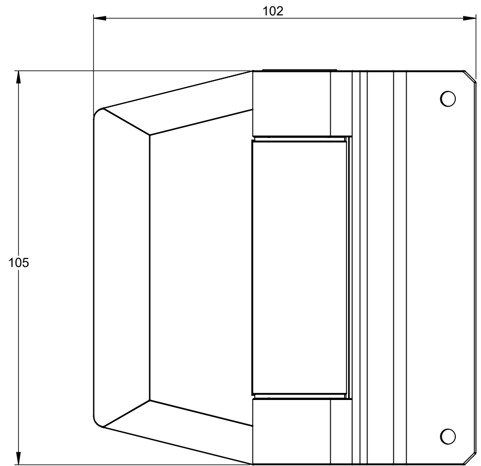
FRONT VIEW
